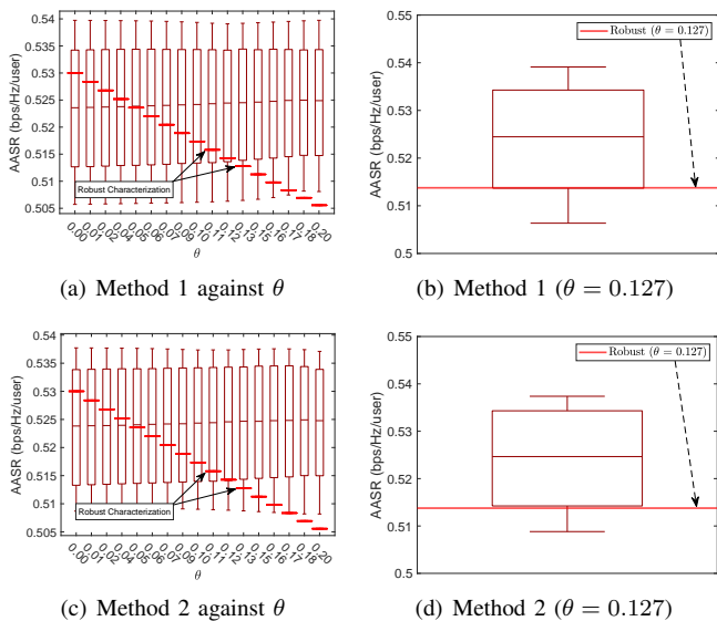
Fig. 7. Conservative characterization under robust sensing-centric waveform design. Red step values show the robust performance characterizations R_{H^*}, \mathbf{X}^* under different \theta . When \theta \approx 0.127 , R_{H^*}, \mathbf{X}^* correctly identifies the tightest conservative performance bounds of true AASRs, with probability 95%. NB: \theta = 0 gives nominal characterizations. (Cf. Fig. 2(b).)
